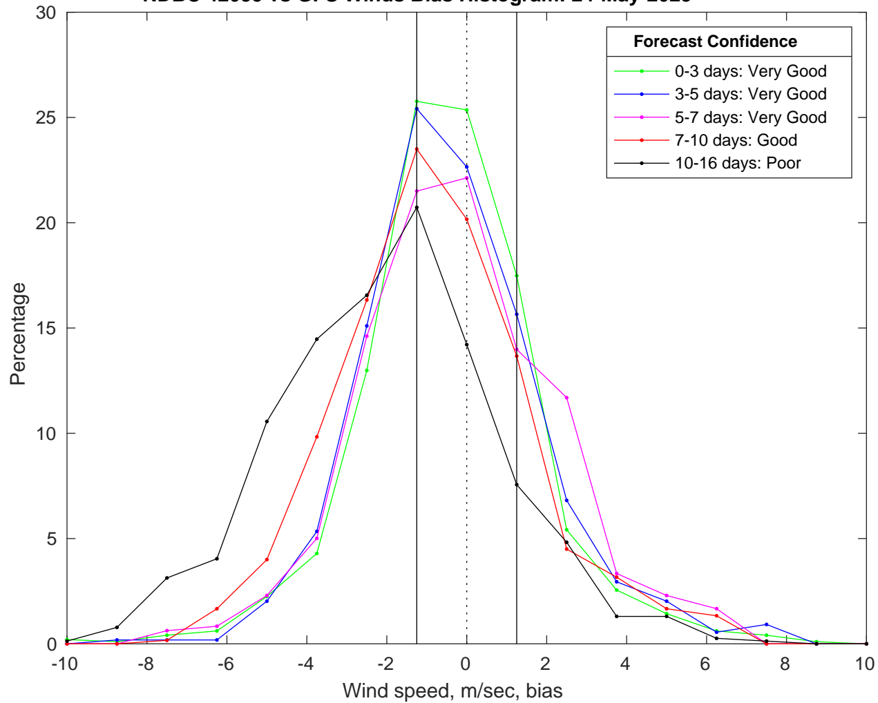
NDBC 42035 vs GFS Winds Bias Histogram: 24-May-2025
