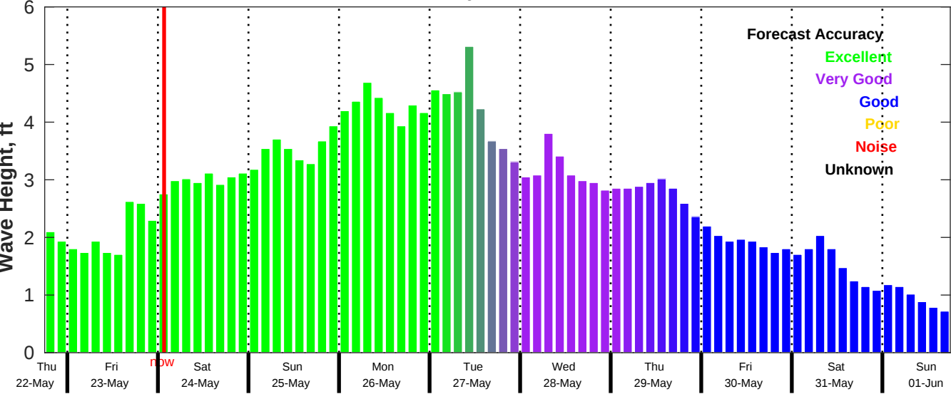
CMEMS Wave Forecast for NDBC 42035 from 22-May-2025 18:00:00 to 01-Jun-2025 18:00:00
