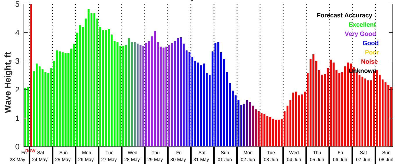
GFS Wave Forecast for NDBC 42035 from 23-May-2025 18:00:00 to 08-Jun-2025 18:00:00
