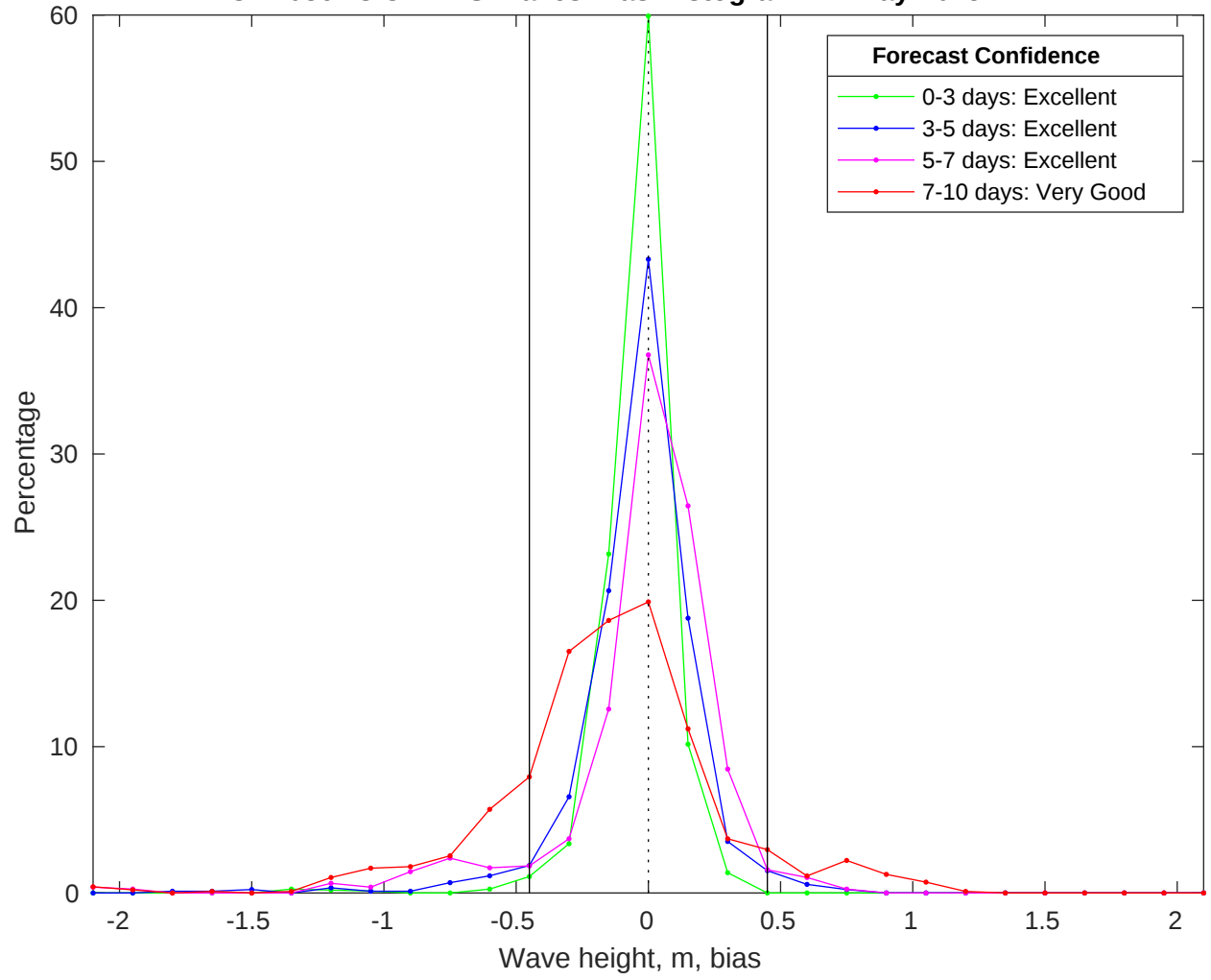
NDBC 42036 vs CMEMS Waves Bias Histogram: 24-May-2025
