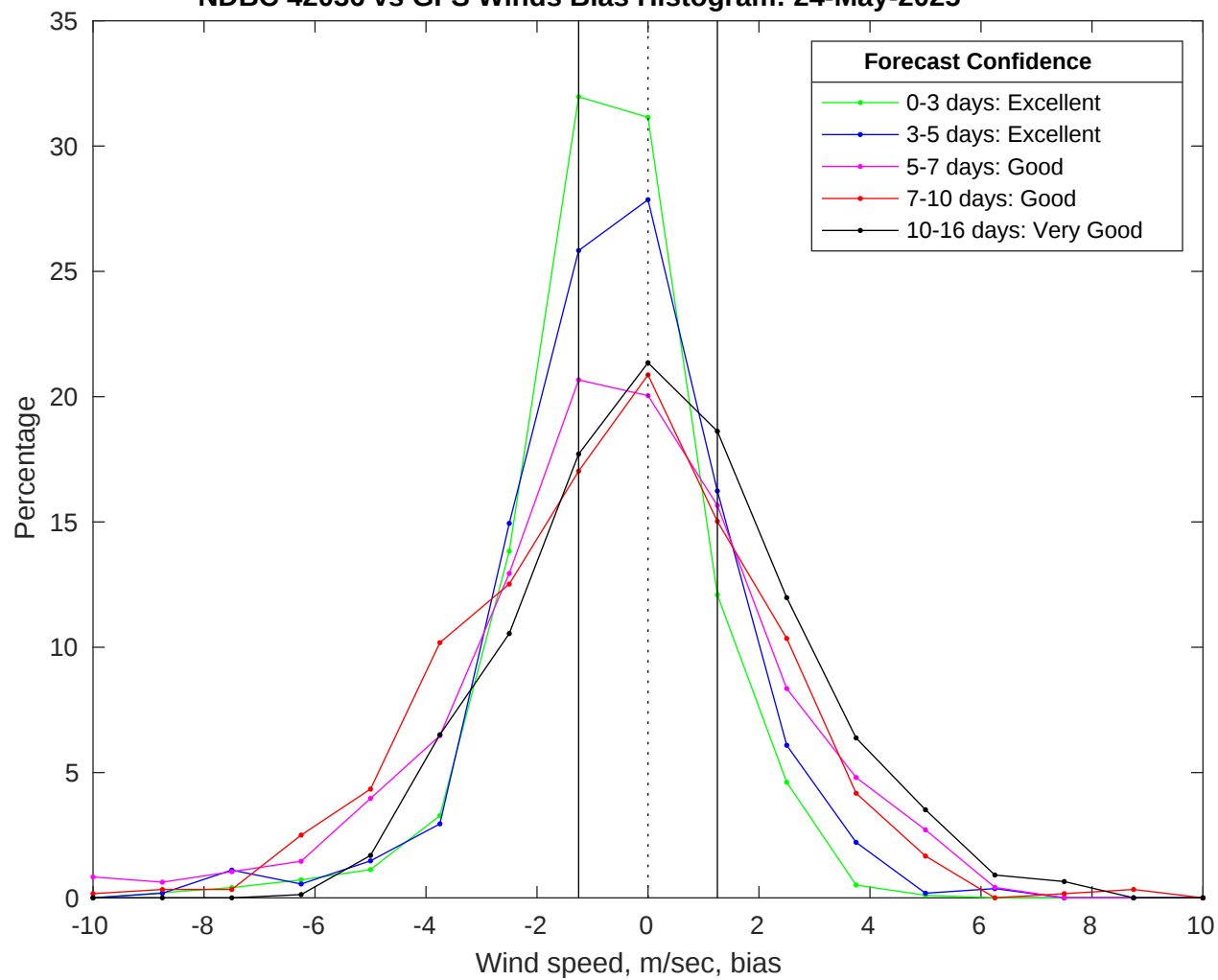
NDBC 42036 vs GFS Winds Bias Histogram: 24-May-2025
