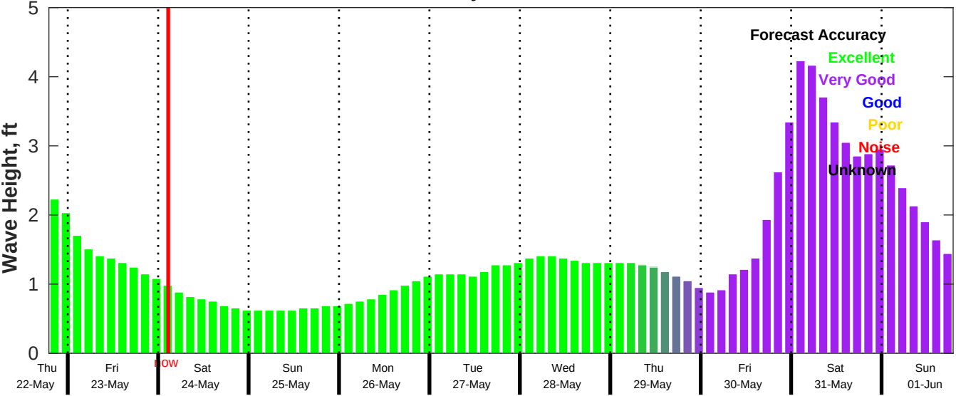
CMEMS Wave Forecast for NDBC 42036 from 22-May-2025 19:00:00 to 01-Jun-2025 19:00:00
