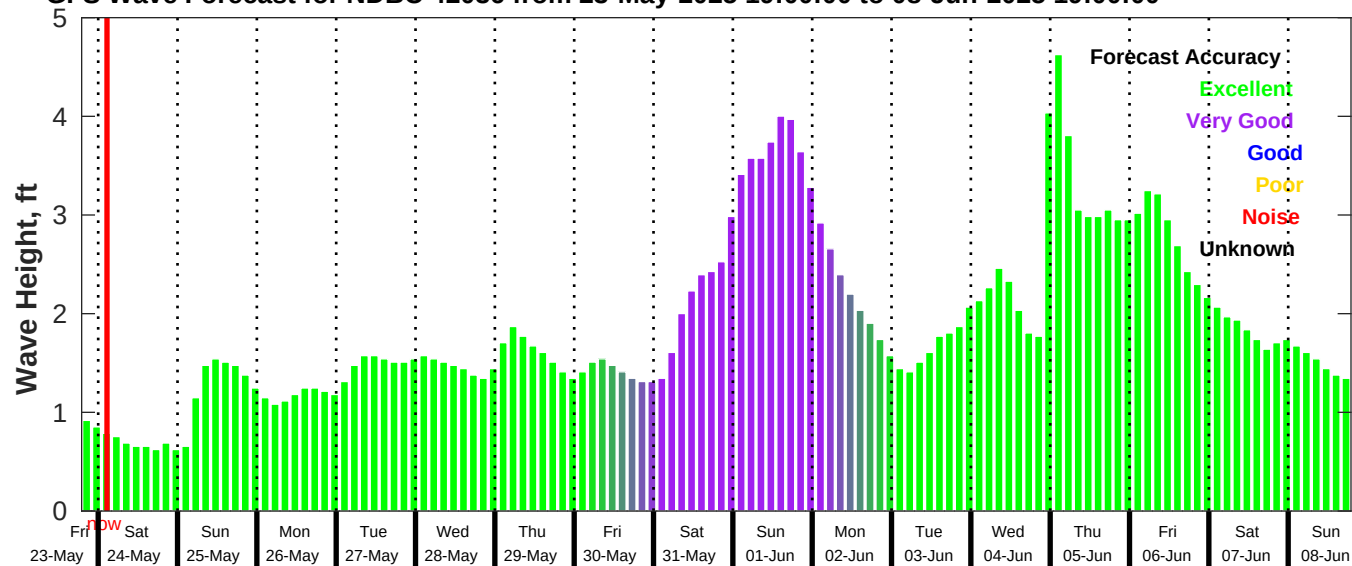
GFS Wave Forecast for NDBC 42036 from 23-May-2025 19:00:00 to 08-Jun-2025 19:00:00
