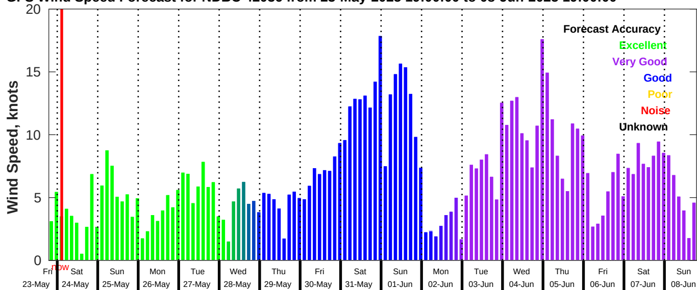
GFS Wind Speed Forecast for NDBC 42036 from 23-May-2025 19:00:00 to 08-Jun-2025 19:00:00
