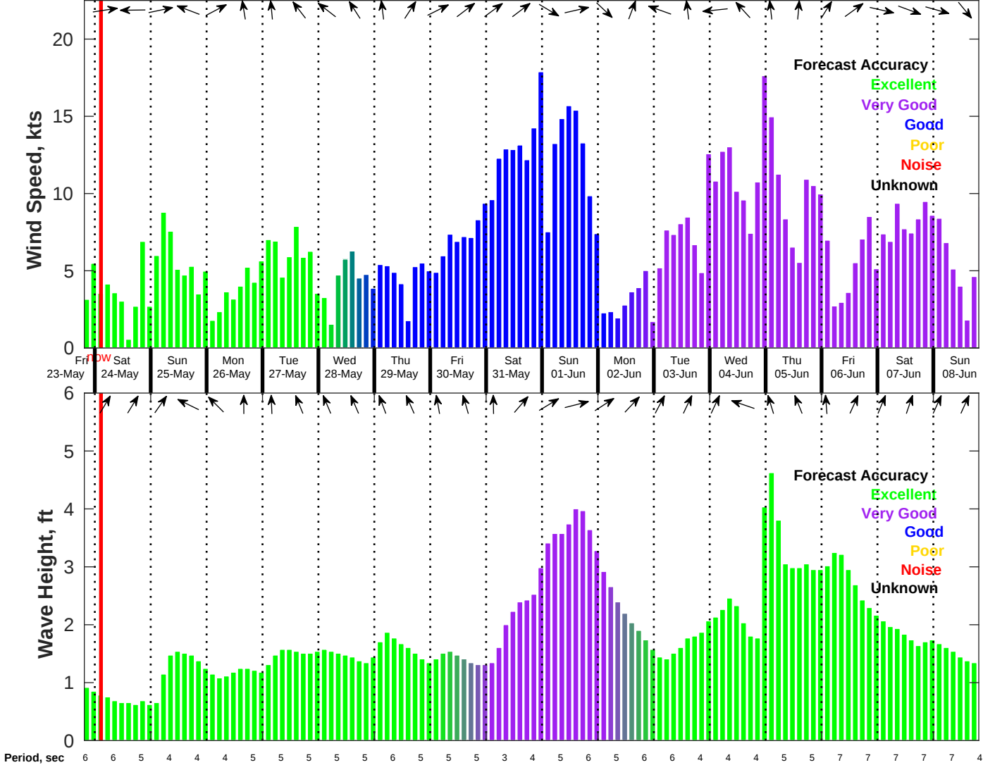
Wind & Wave Forecast for NDBC 42036 from 23-May-2025 19:00:00 to 08-Jun-2025 19:00:00
