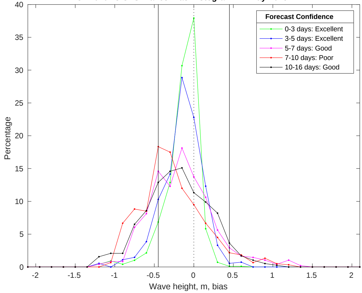
NDBC 42040 vs GFS Waves Bias Histogram: 24-May-2025
