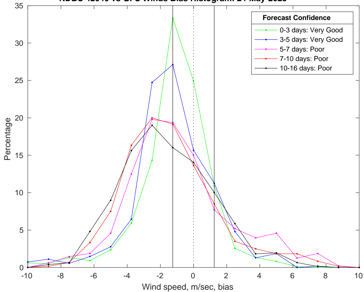
NDBC 42040 vs GFS Winds Bias Histogram: 24-May-2025
