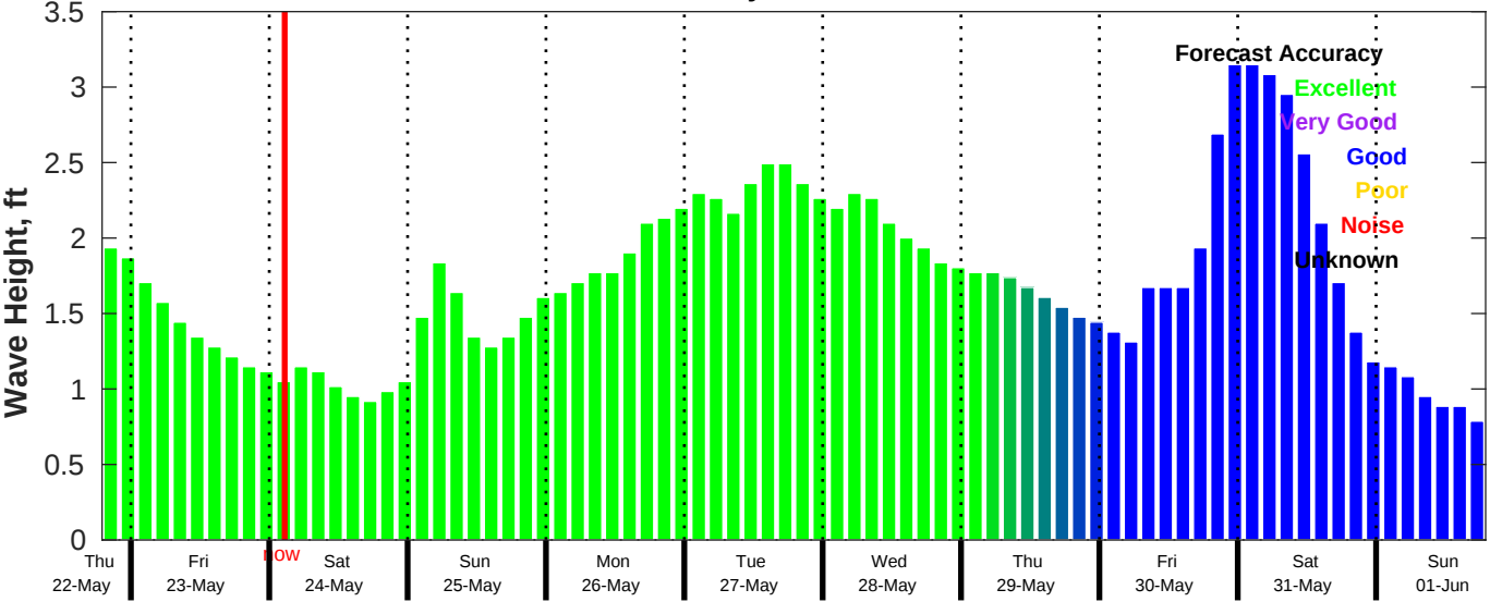
CMEMS Wave Forecast for NDBC 42040 from 22-May-2025 19:00:00 to 01-Jun-2025 19:00:00
