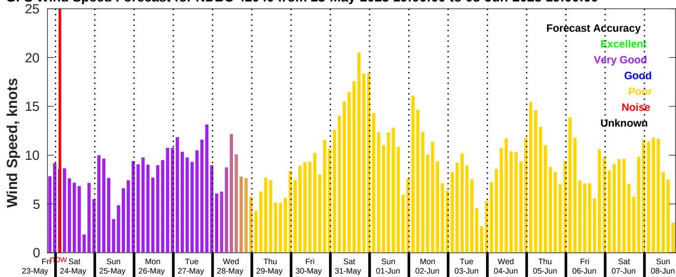
GFS Wind Speed Forecast for NDBC 42040 from 23-May-2025 19:00:00 to 08-Jun-2025 19:00:00
