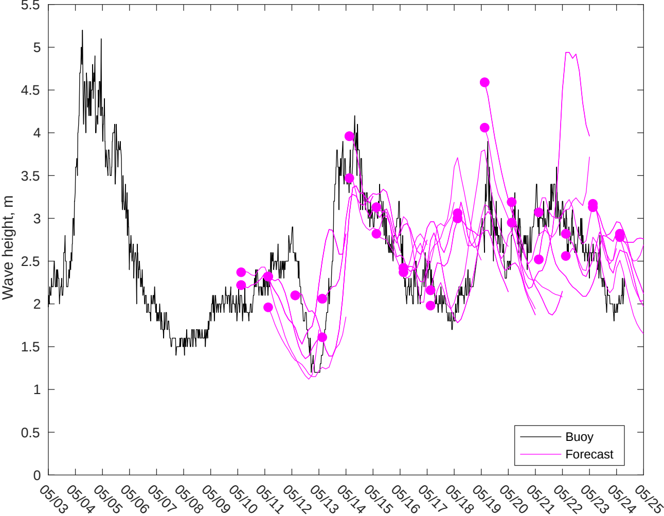
NDBC 46011 vs CMEMS Waves: 7 to 10 day forecast
