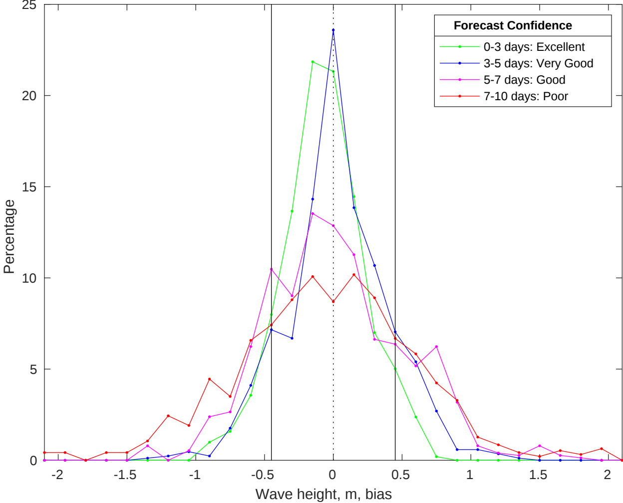
NDBC 46011 vs CMEMS Waves Bias Histogram: 24-May-2025
