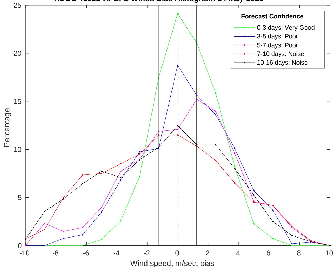
NDBC 46011 vs GFS Winds Bias Histogram: 24-May-2025
