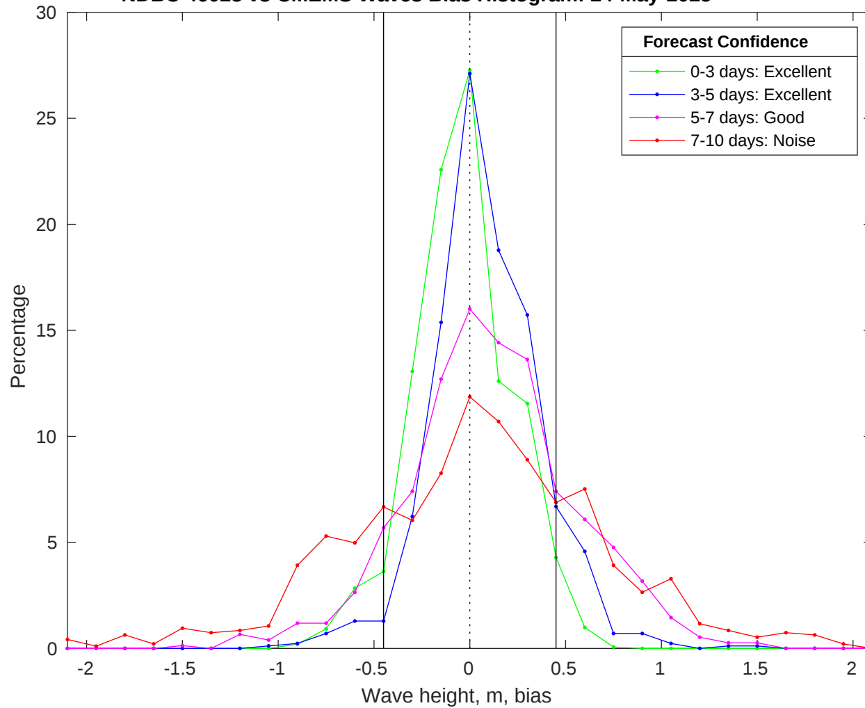
NDBC 46028 vs CMEMS Waves Bias Histogram: 24-May-2025
