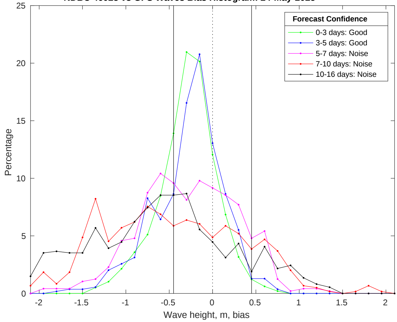
NDBC 46028 vs GFS Waves Bias Histogram: 24-May-2025
