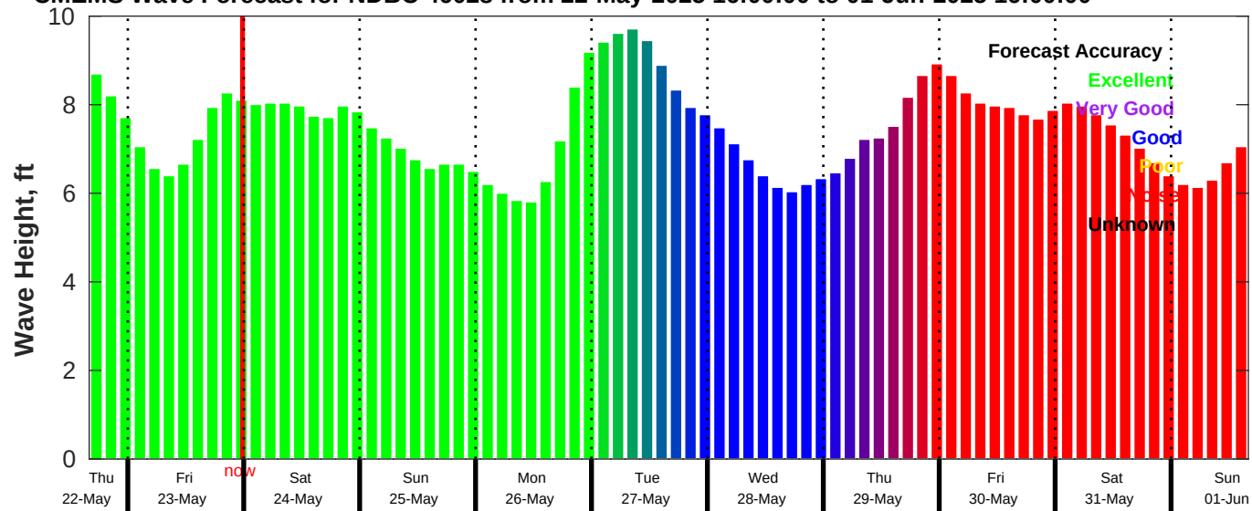
CMEMS Wave Forecast for NDBC 46028 from 22-May-2025 16:00:00 to 01-Jun-2025 16:00:00
