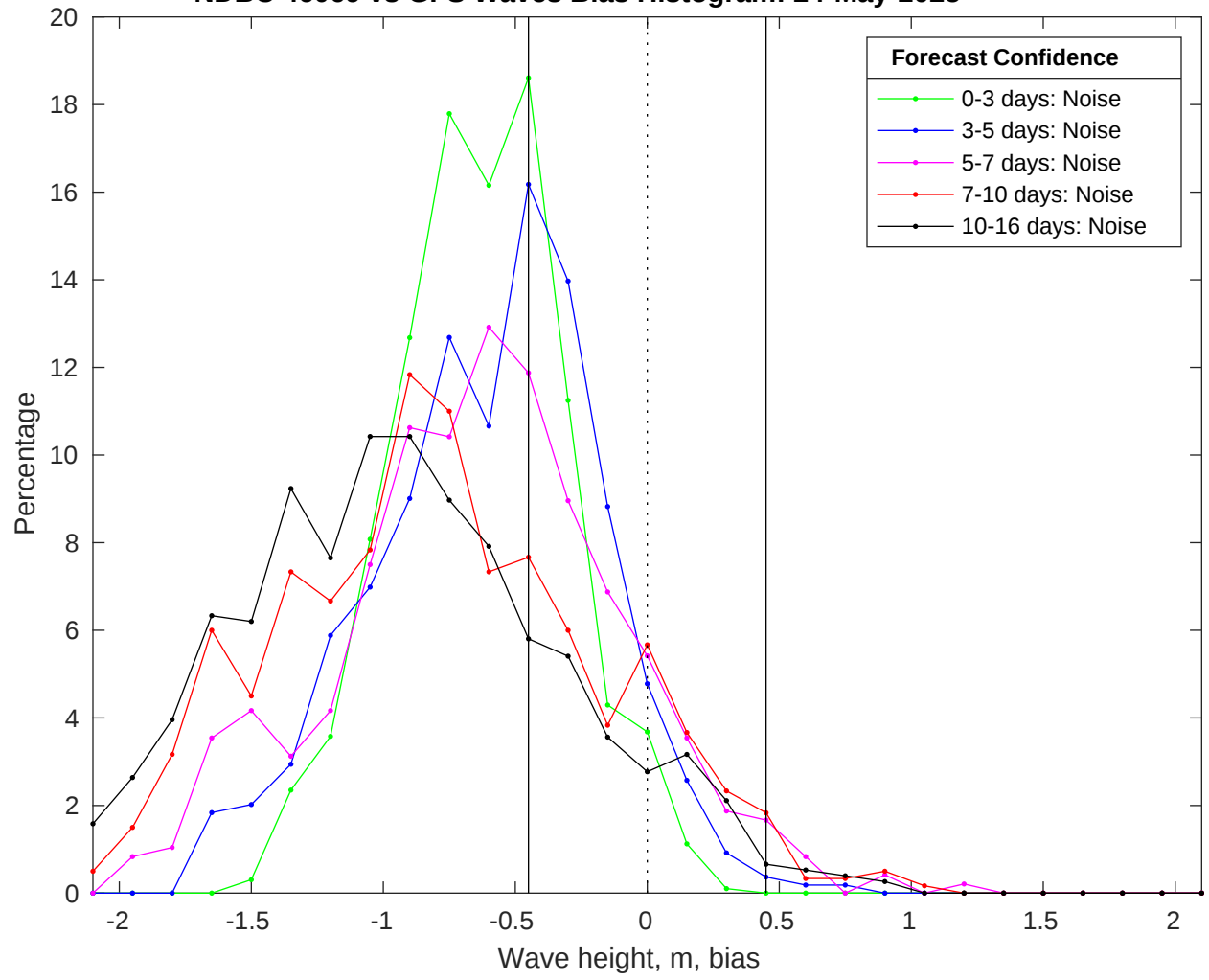
NDBC 46069 vs GFS Waves Bias Histogram: 24-May-2025
