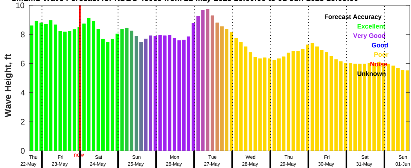
CMEMS Wave Forecast for NDBC 46069 from 22-May-2025 16:00:00 to 01-Jun-2025 16:00:00
