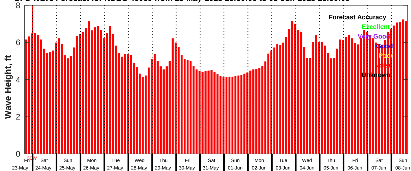
GFS Wave Forecast for NDBC 46069 from 23-May-2025 16:00:00 to 08-Jun-2025 16:00:00
