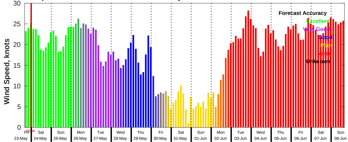
GFS Wind Speed Forecast for NDBC 46069 from 23-May-2025 16:00:00 to 08-Jun-2025 16:00:00
