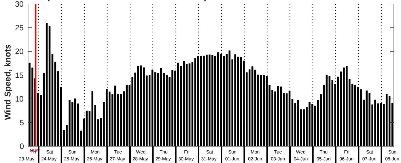
GFS Wind Speed Forecast for NDBC 51209 from 23-May-2025 13:00:00 to 08-Jun-2025 13:00:00
