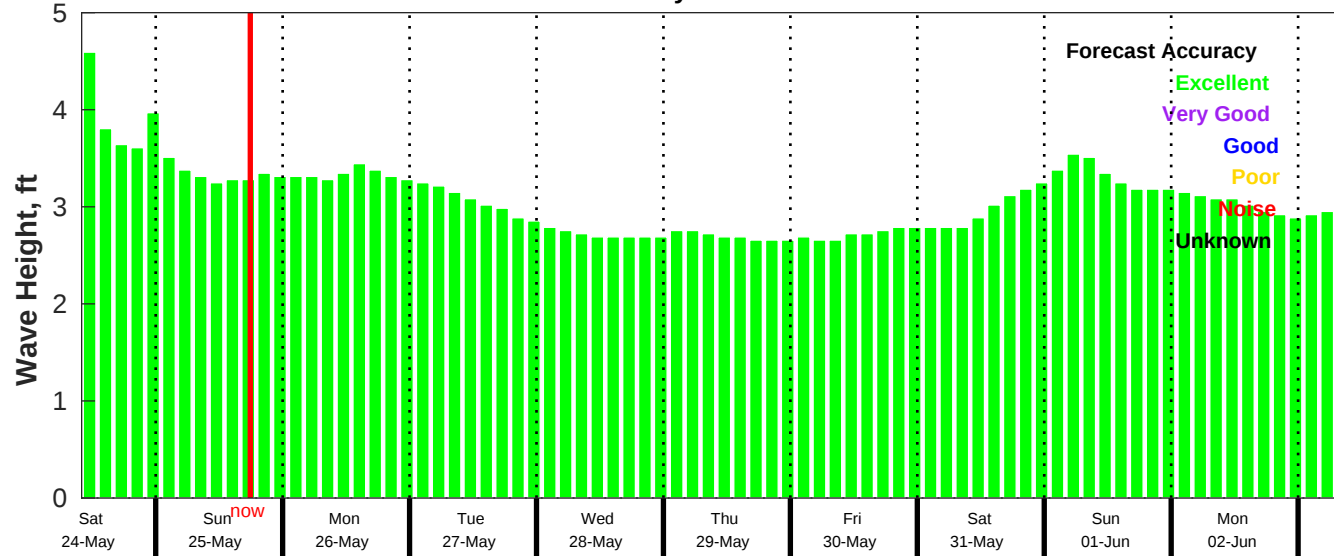
CMEMS Wave Forecast for NDBC 52211 from 23-May-2025 10:00:00 to 02-Jun-2025 10:00:00
