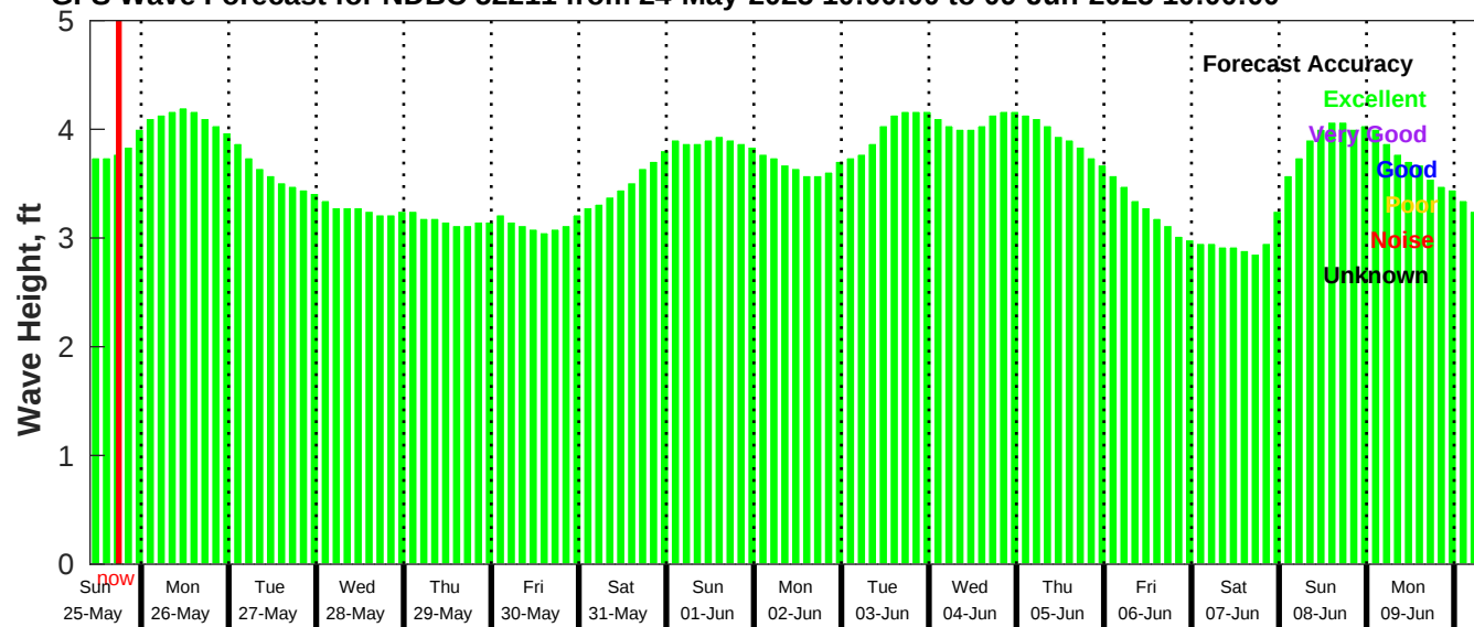
GFS Wave Forecast for NDBC 52211 from 24-May-2025 10:00:00 to 09-Jun-2025 10:00:00
