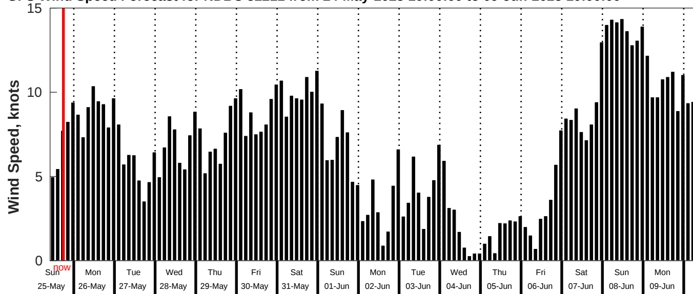
GFS Wind Speed Forecast for NDBC 52211 from 24-May-2025 10:00:00 to 09-Jun-2025 10:00:00
