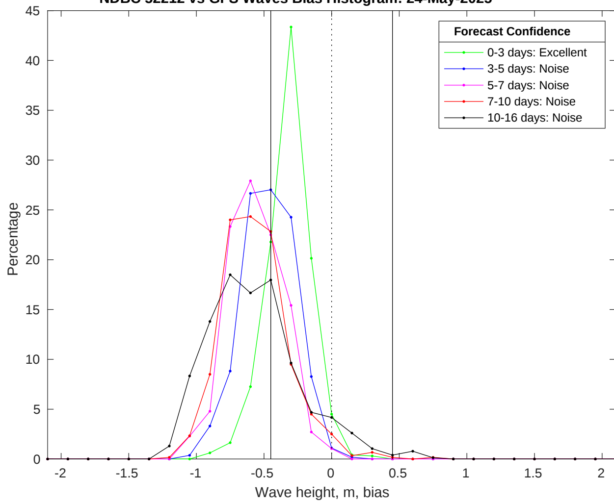
NDBC 52212 vs GFS Waves Bias Histogram: 24-May-2025
