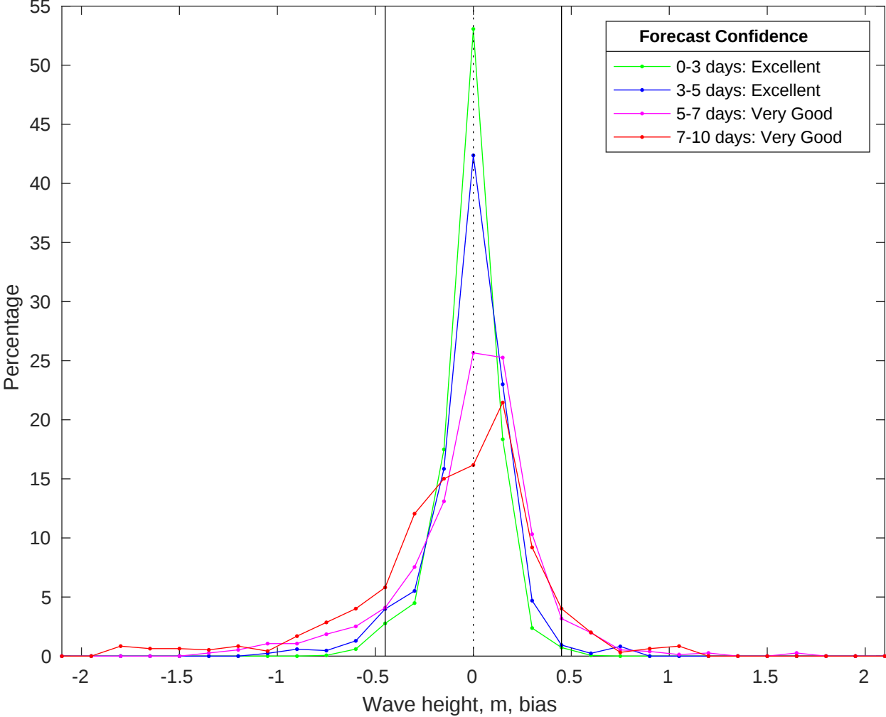
NDBC 41004 vs CMEMS Waves Bias Histogram: 25-May-2025
