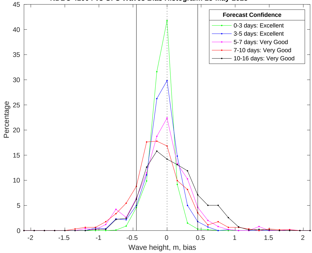
NDBC 41004 vs GFS Waves Bias Histogram: 25-May-2025
