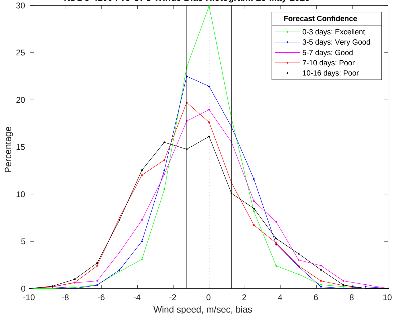
NDBC 41004 vs GFS Winds Bias Histogram: 25-May-2025
