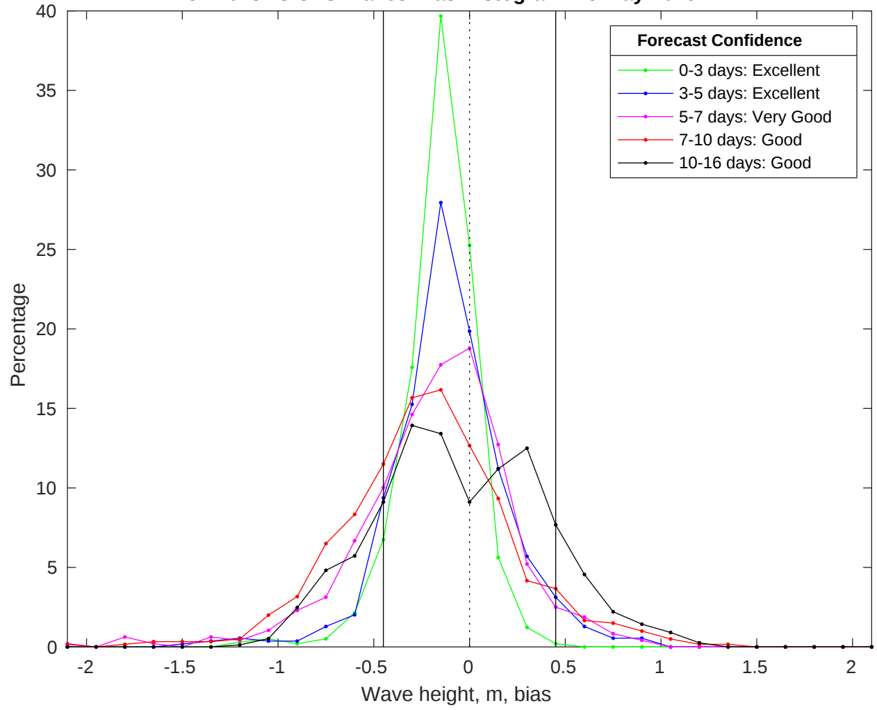
NDBC 41013 vs GFS Waves Bias Histogram: 25-May-2025
