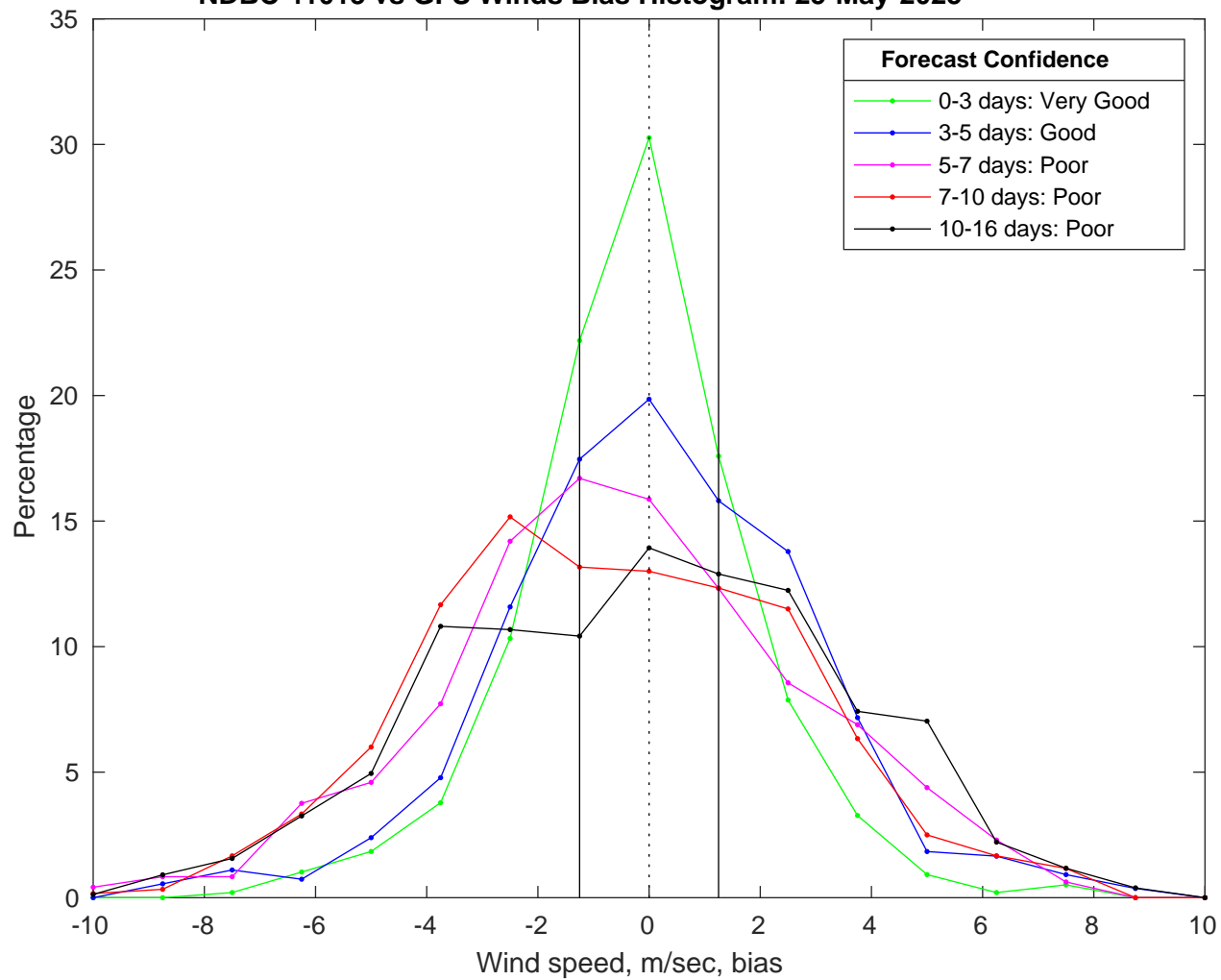
NDBC 41013 vs GFS Winds Bias Histogram: 25-May-2025
