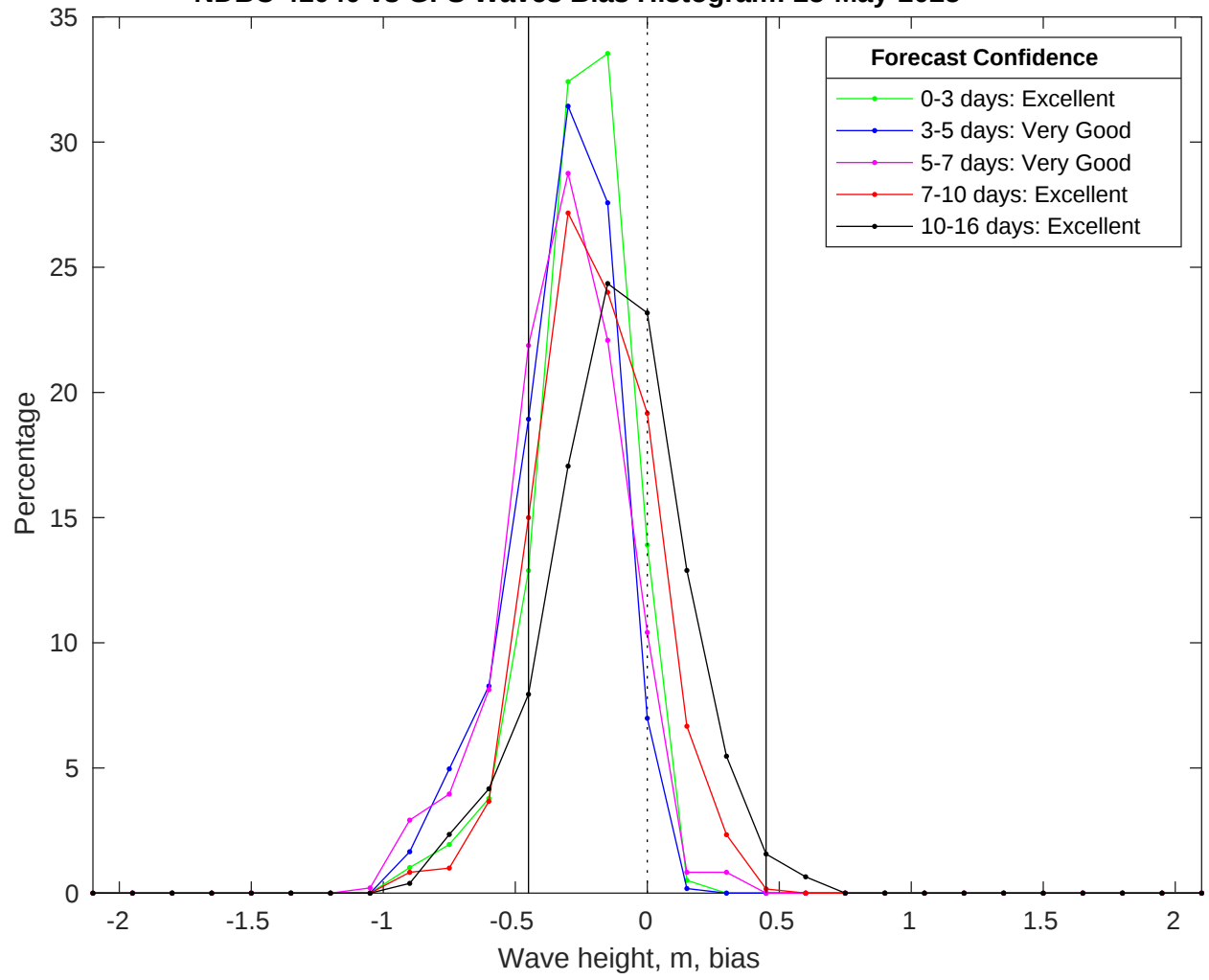
NDBC 41040 vs GFS Waves Bias Histogram: 25-May-2025
