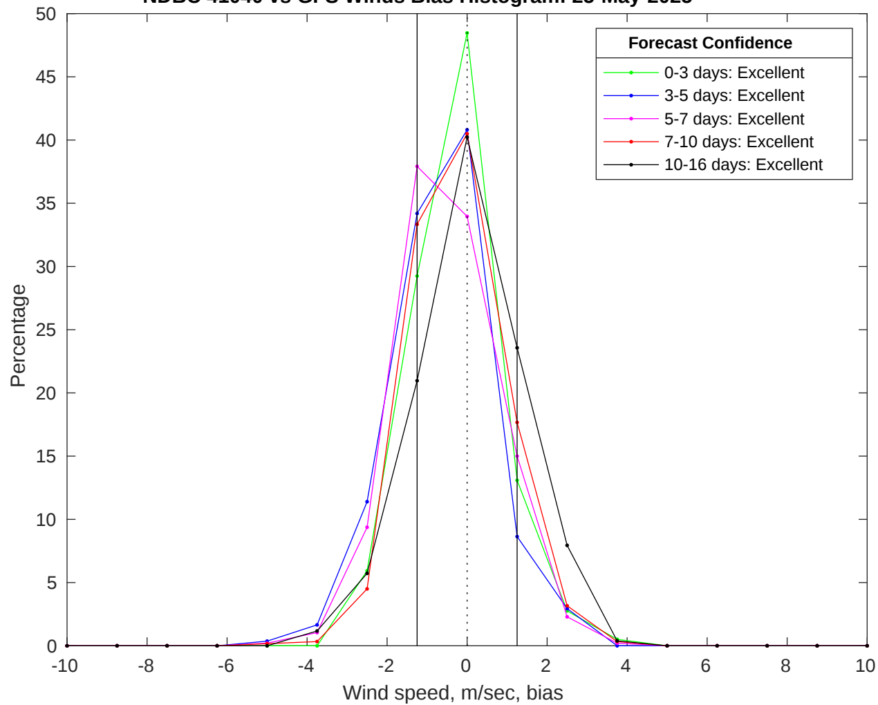
NDBC 41040 vs GFS Winds Bias Histogram: 25-May-2025
