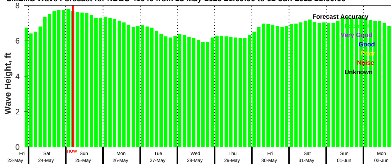
CMEMS Wave Forecast for NDBC 41040 from 23-May-2025 21:00:00 to 02-Jun-2025 21:00:00
