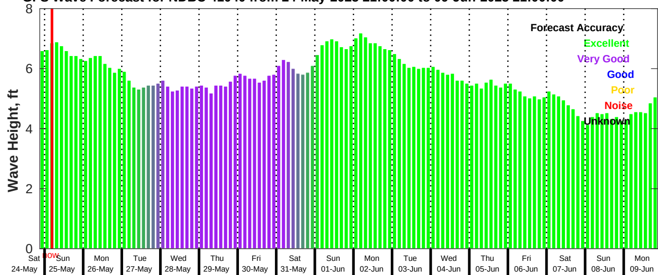
GFS Wave Forecast for NDBC 41040 from 24-May-2025 21:00:00 to 09-Jun-2025 21:00:00
