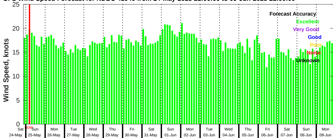
GFS Wind Speed Forecast for NDBC 41040 from 24-May-2025 21:00:00 to 09-Jun-2025 21:00:00
