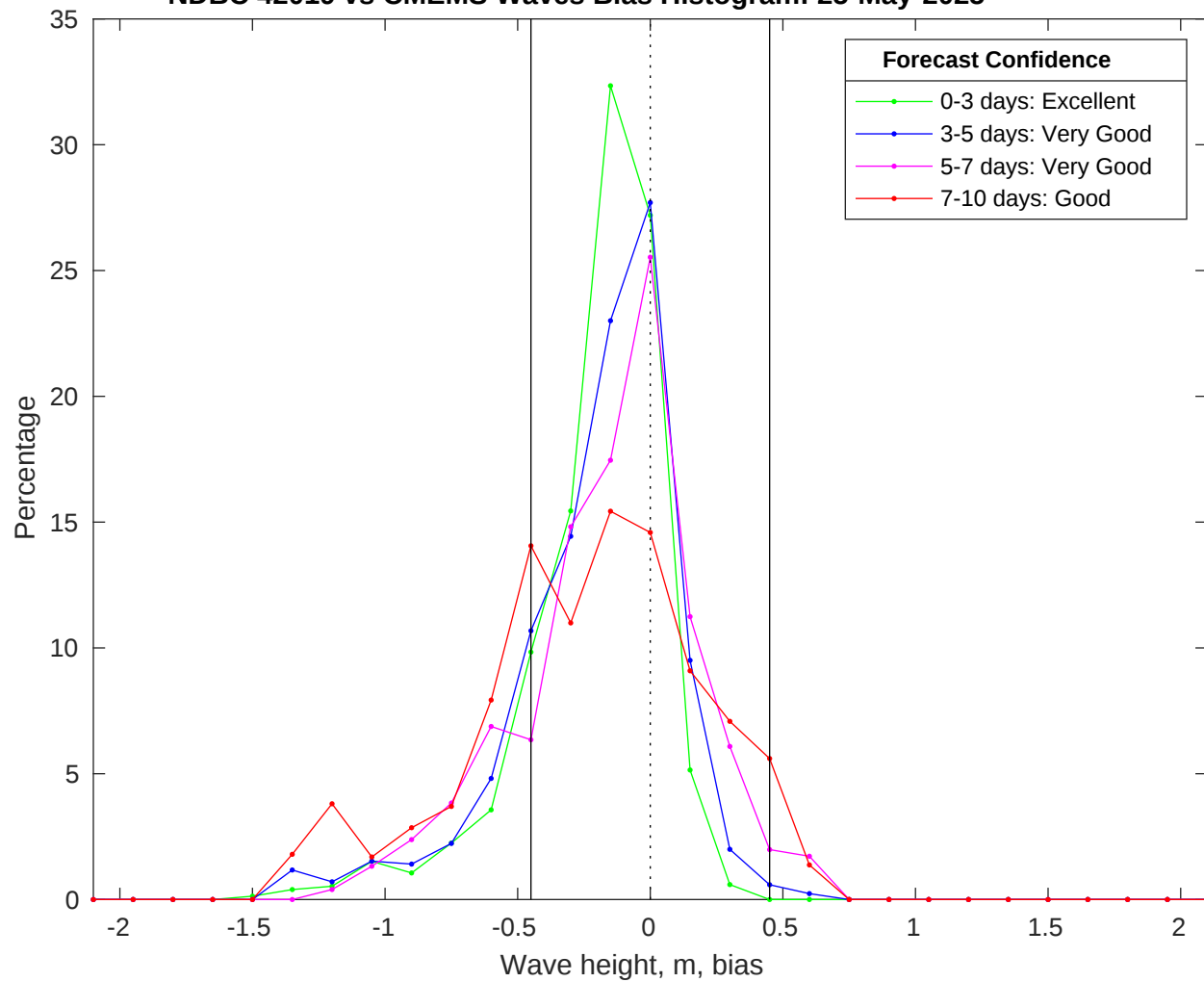
NDBC 42019 vs CMEMS Waves Bias Histogram: 25-May-2025
