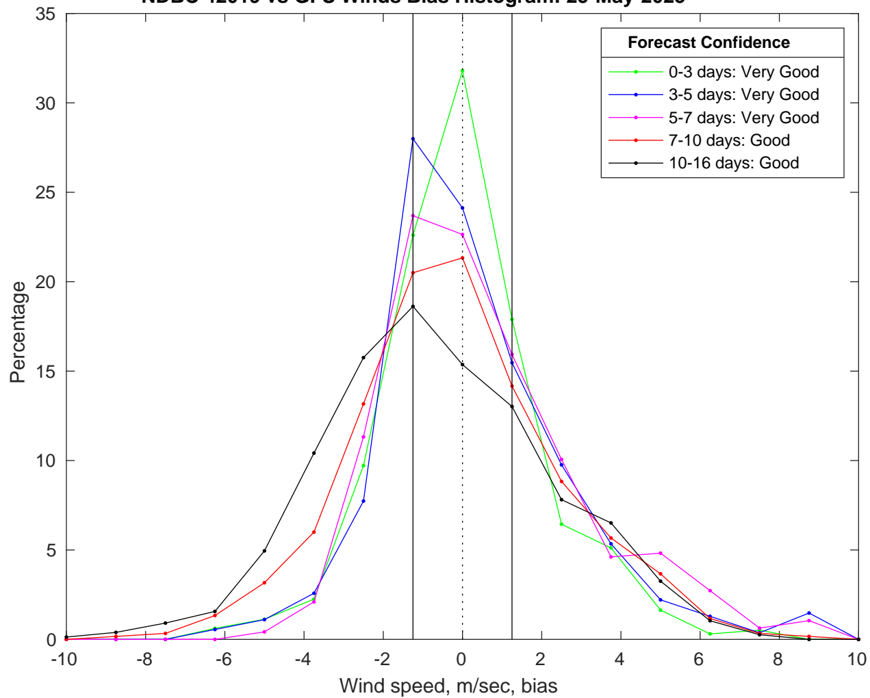
NDBC 42019 vs GFS Winds Bias Histogram: 25-May-2025
