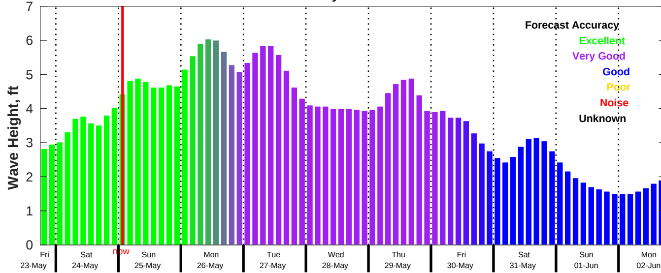
CMEMS Wave Forecast for NDBC 42019 from 23-May-2025 18:00:00 to 02-Jun-2025 18:00:00
