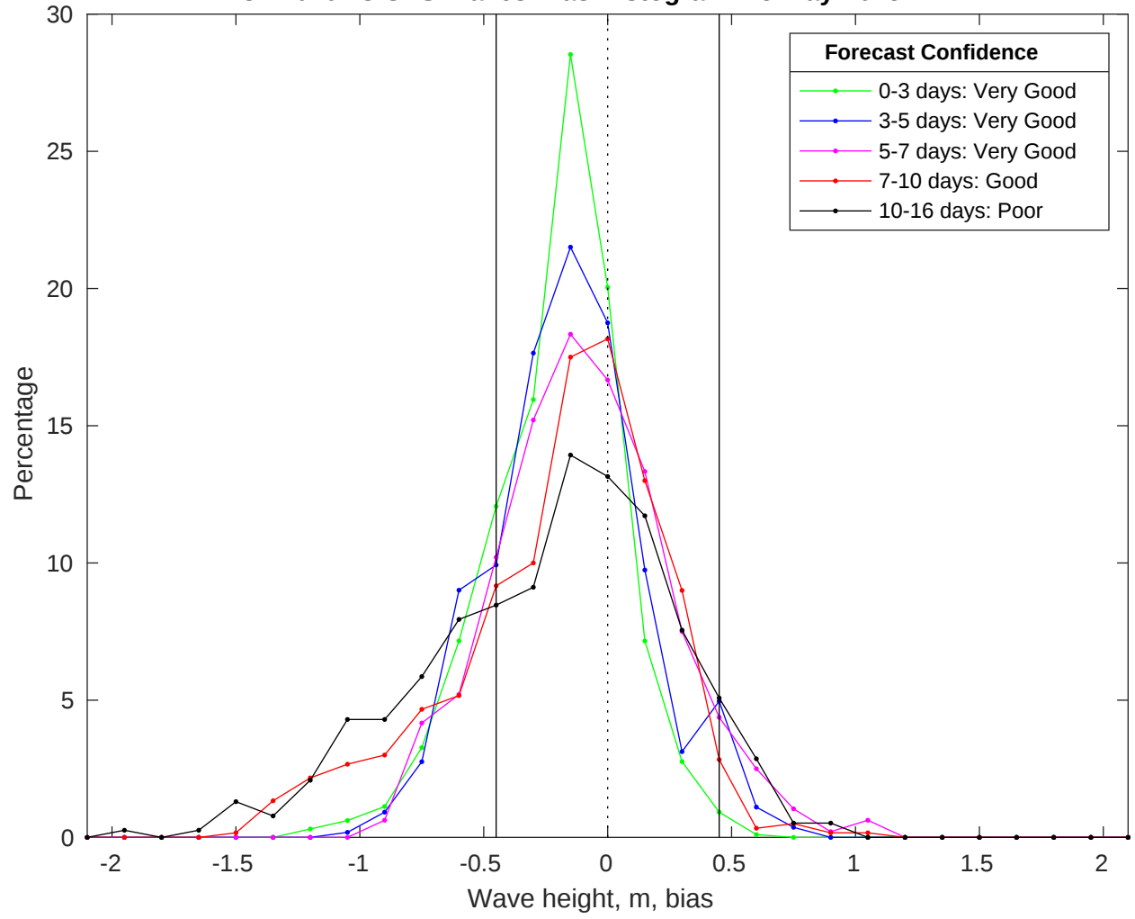
NDBC 42020 vs GFS Waves Bias Histogram: 25-May-2025
