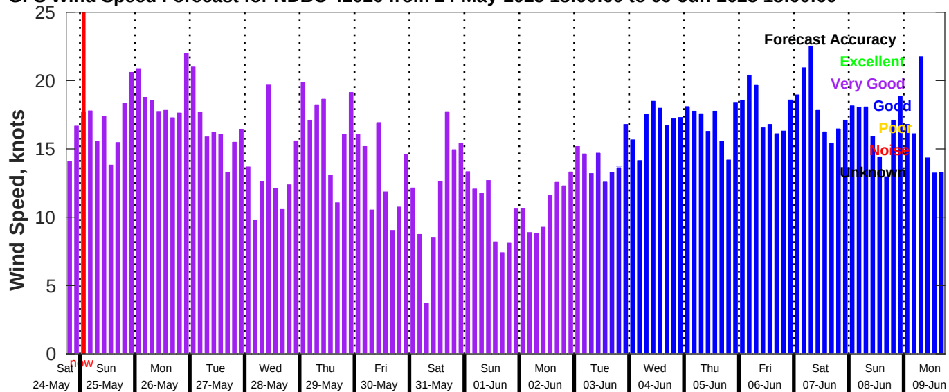
GFS Wind Speed Forecast for NDBC 42020 from 24-May-2025 18:00:00 to 09-Jun-2025 18:00:00
