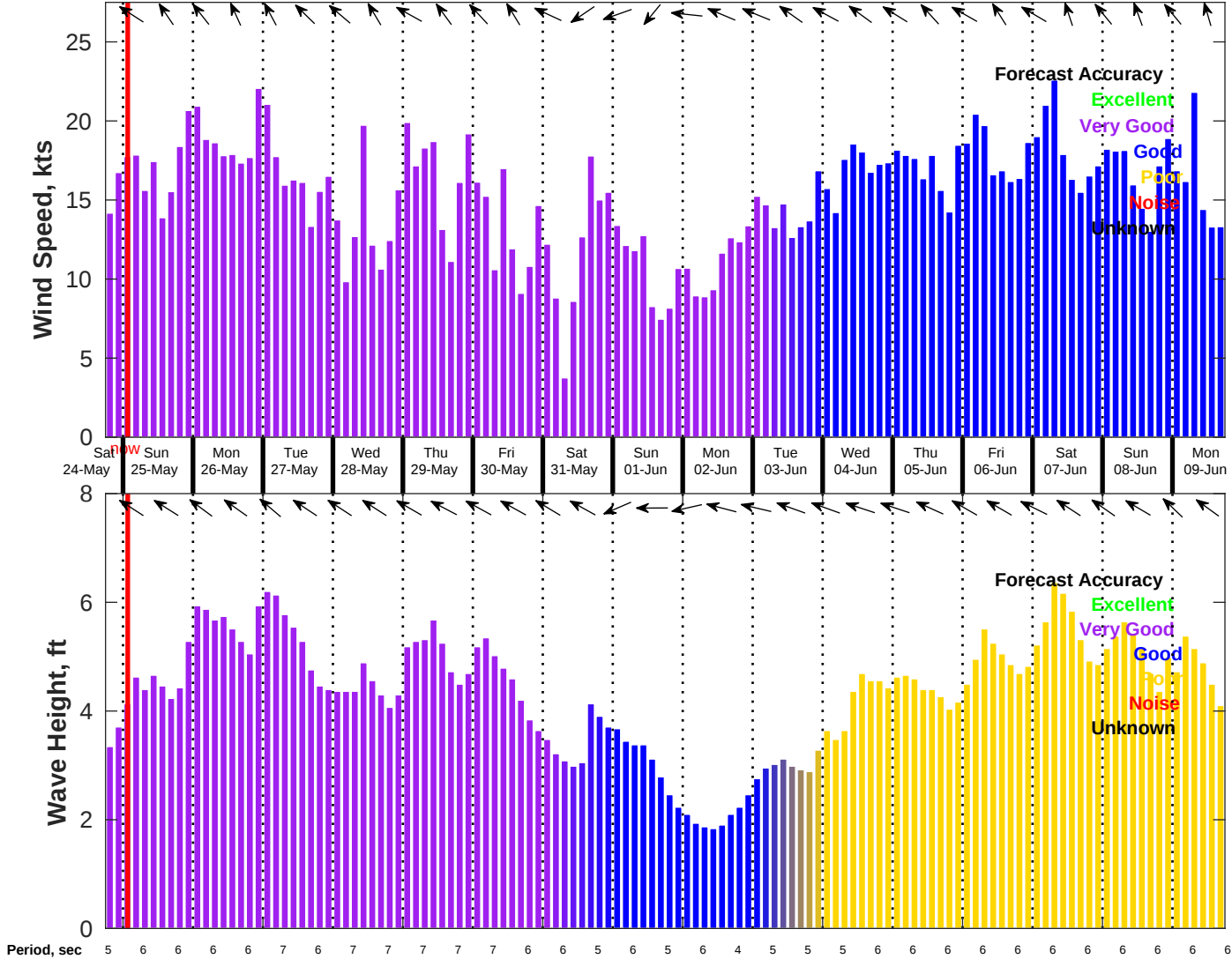
Wind & Wave Forecast for NDBC 42020 from 24-May-2025 18:00:00 to 09-Jun-2025 18:00:00
