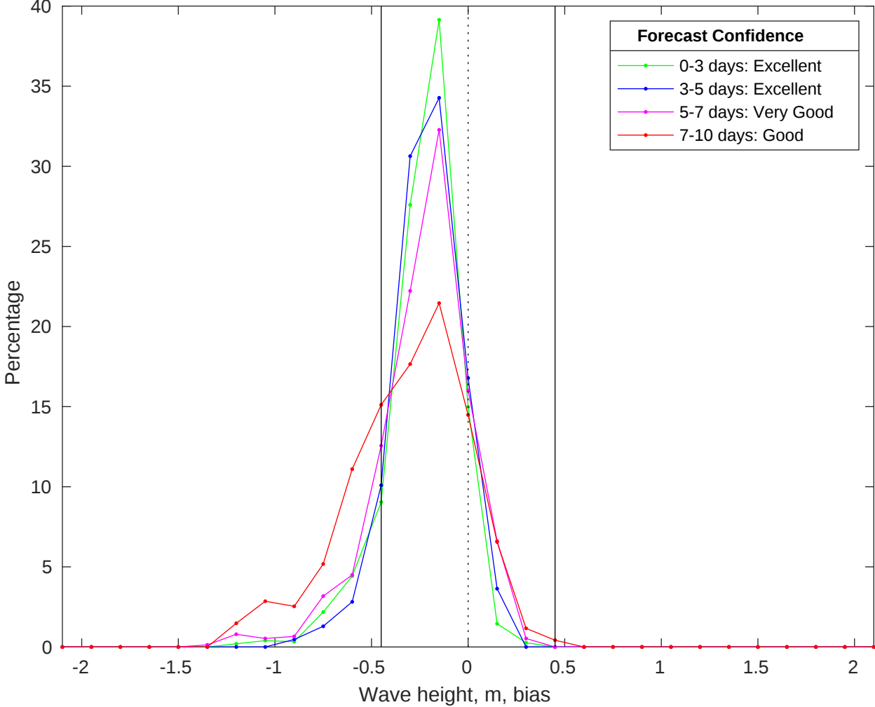
NDBC 42035 vs CMEMS Waves Bias Histogram: 25-May-2025
