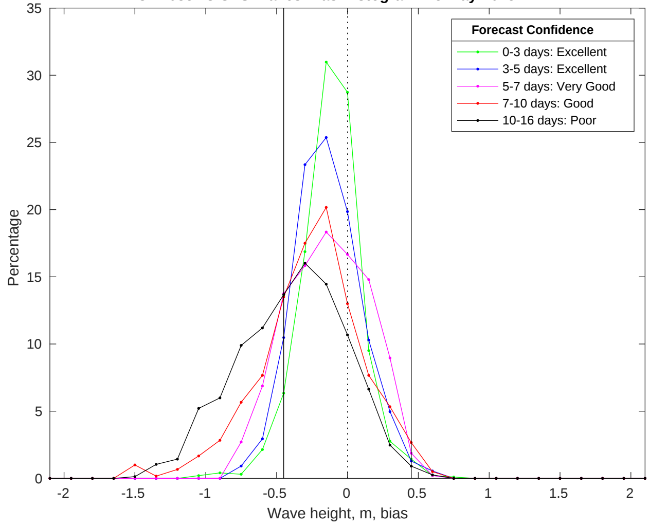
NDBC 42035 vs GFS Waves Bias Histogram: 25-May-2025
