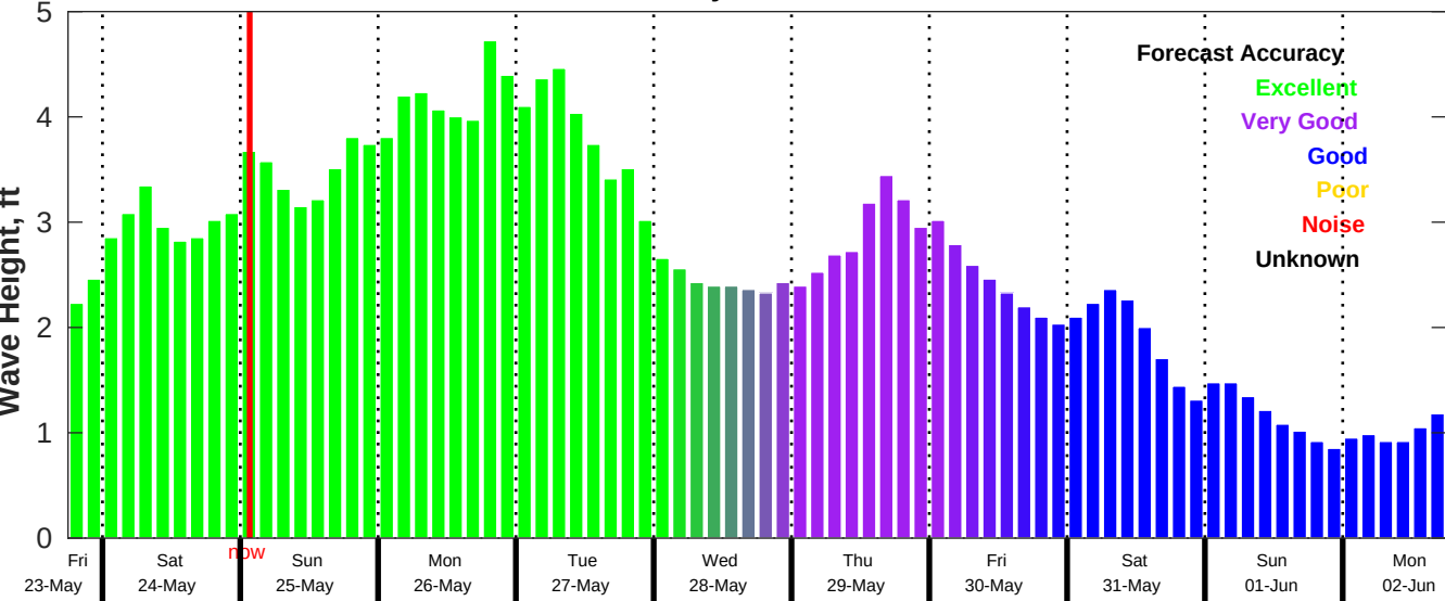
CMEMS Wave Forecast for NDBC 42035 from 23-May-2025 18:00:00 to 02-Jun-2025 18:00:00
