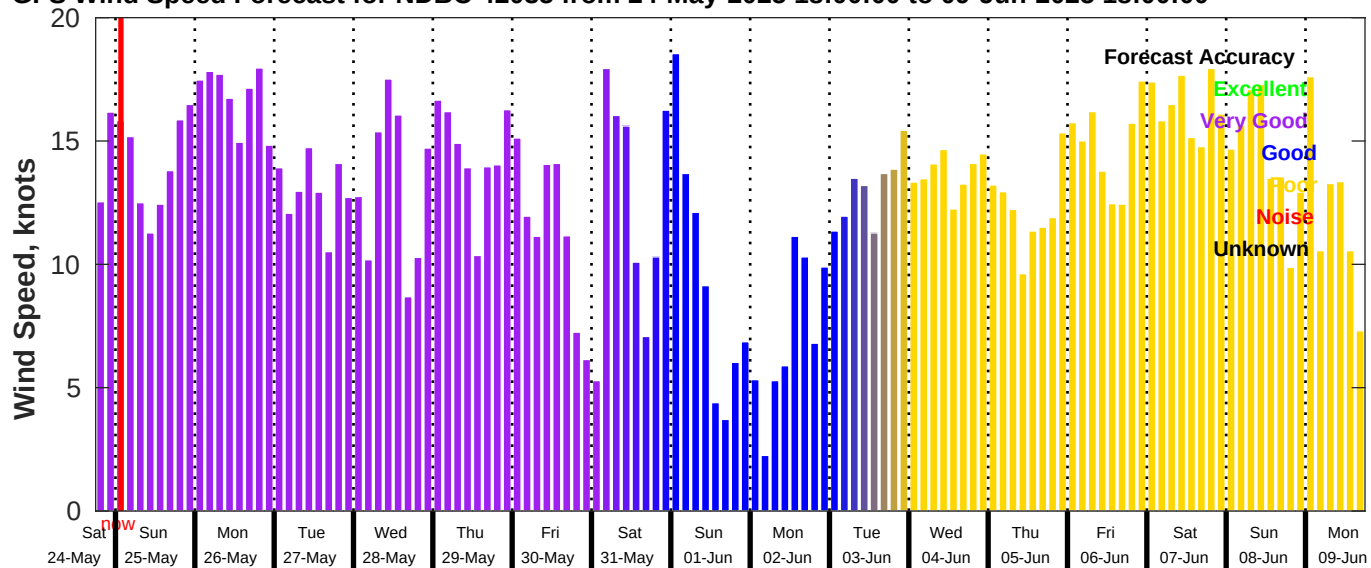
GFS Wind Speed Forecast for NDBC 42035 from 24-May-2025 18:00:00 to 09-Jun-2025 18:00:00
