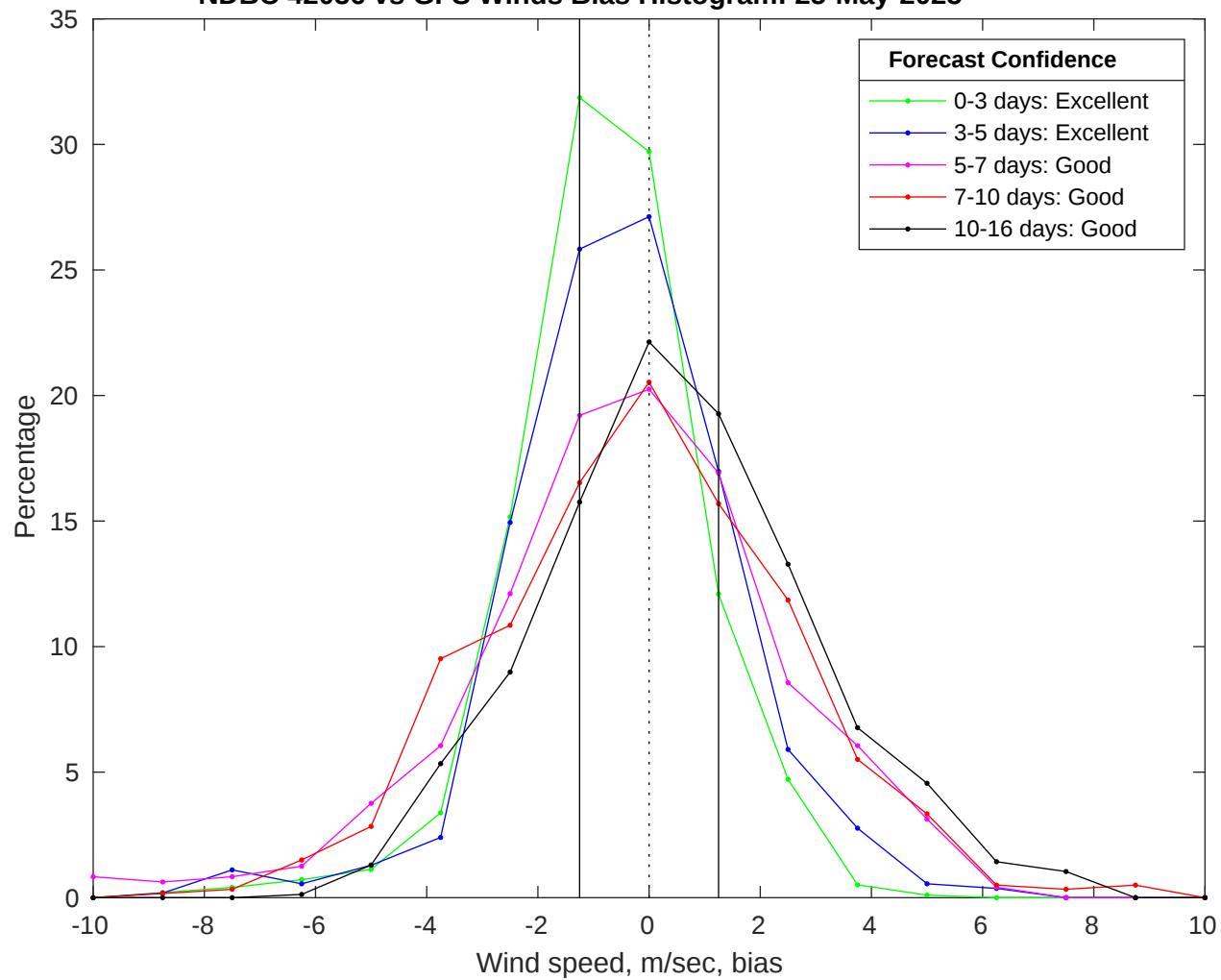
NDBC 42036 vs GFS Winds Bias Histogram: 25-May-2025
