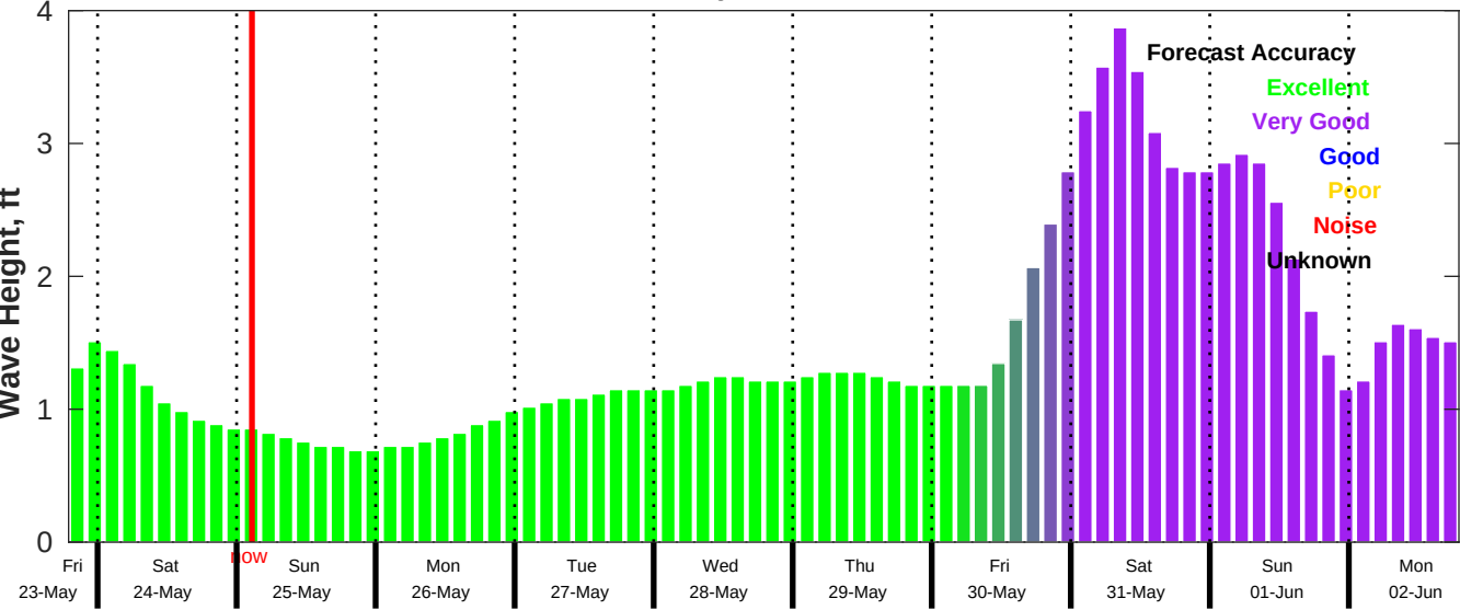
CMEMS Wave Forecast for NDBC 42036 from 23-May-2025 19:00:00 to 02-Jun-2025 19:00:00
